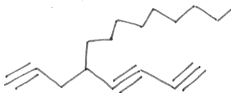
5 nonyl oct-1,3,7-triyne
