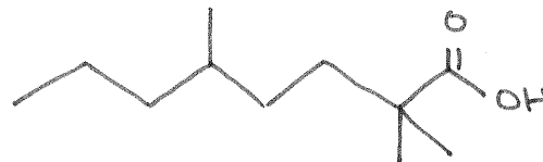
Nonyl ethanoate
