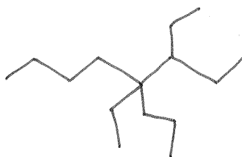
1,2,3,3,4 pentapropyl cycloheptane
