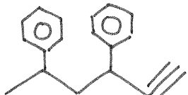
3,5 diphenyl hexyne
